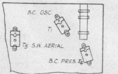
SECTION OF CHASSIS SHOWING TRIMMERS MOUNTED UNDERNEATH
